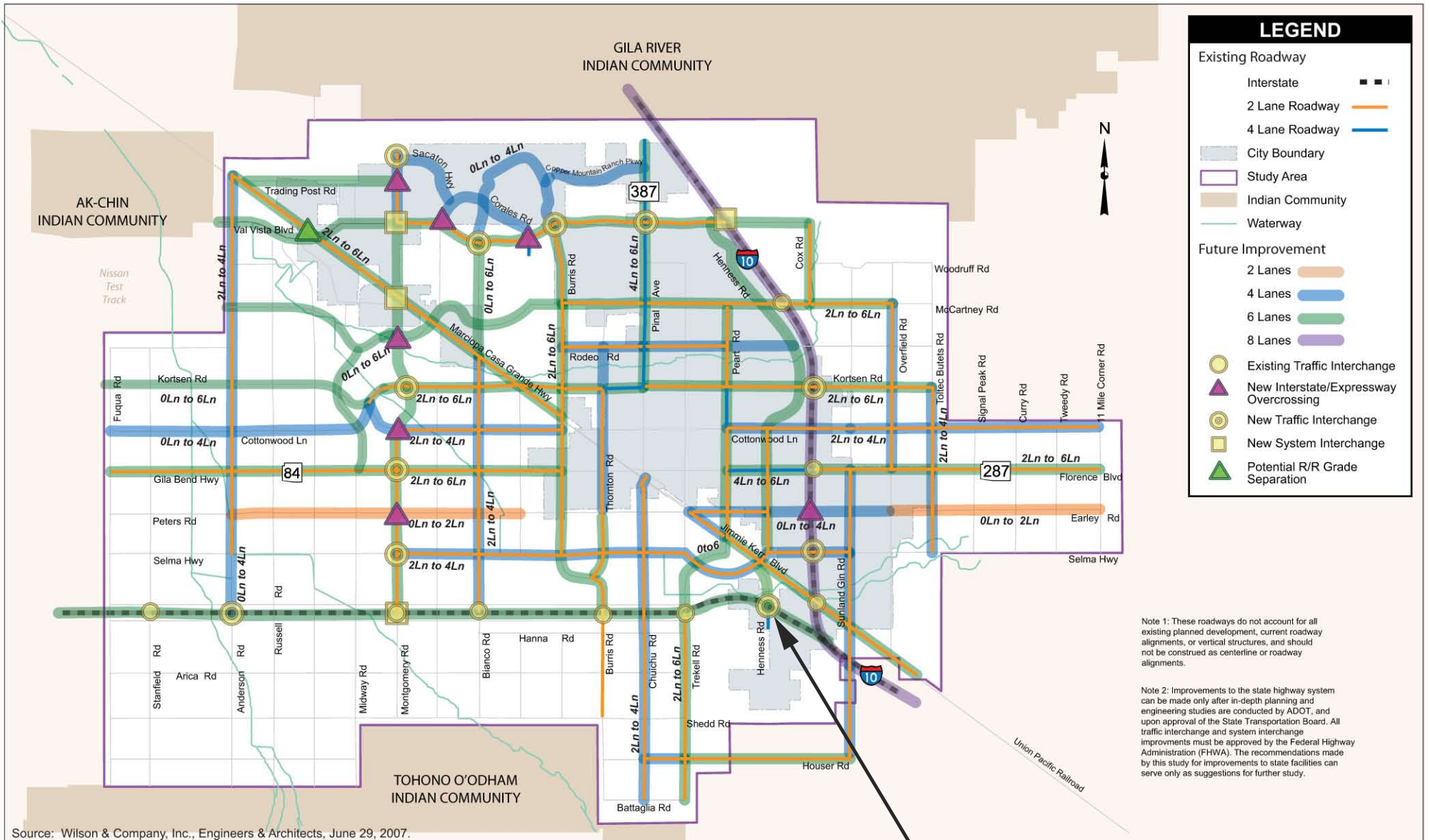
FIGURE 6-2 Year 2030 Roadway Improvement Plan
